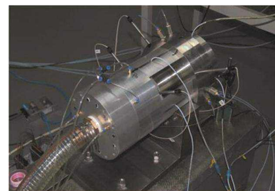
rotor test bench
